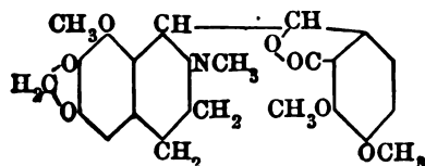
Narcotine.
